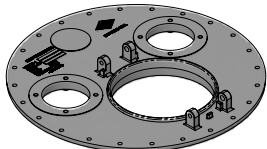
VOH501E VOH501E-1 WITHOUT PROBE MOUNT
