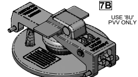
VOH501-33B OPERABLE BRIDGE, LOCKABLE HANDLE AND EMERGENCY VENT SUB-ASSEMBLY
