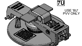
VOH501-33U OPERABLE BRIDGE, LOCKABLE HANDLE AND EMERGENCY VENT SUB-ASSEMBLY
