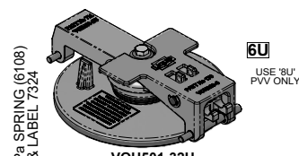
VOH501-32U OPERABLE BRIDGE, PLAIN HANDLE AND EMERGENCY VENT SUB-ASSEMBLY
