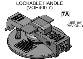
VOH501-33A OPERABLE BRIDGE, LOCKABLE HANDLE AND EMERGENCY VENT SUB-ASSEMBLY
